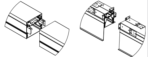
Drywall joining
